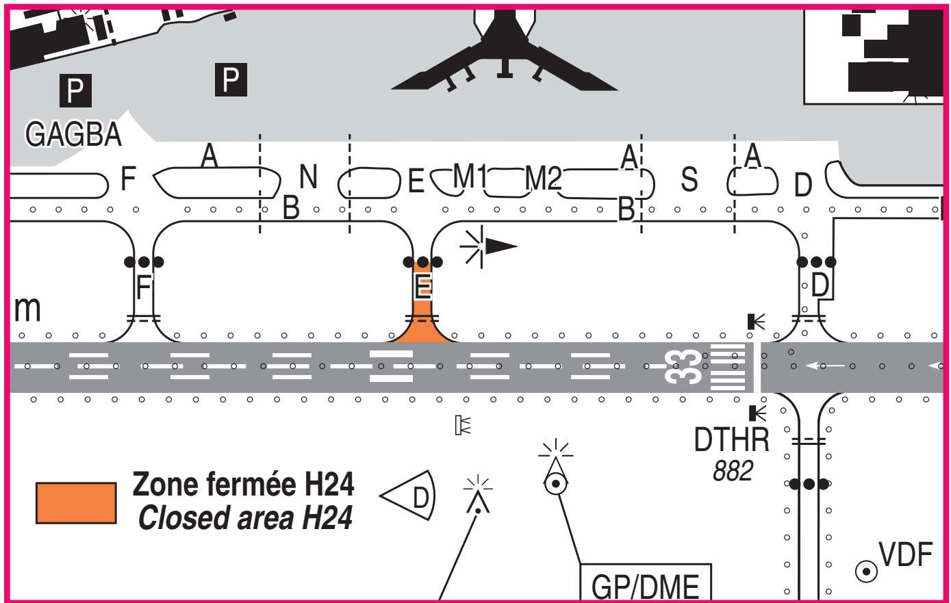
Extrait from AIP France AD 2 LFSB APDC 01 WEF 27 FEB 2020
