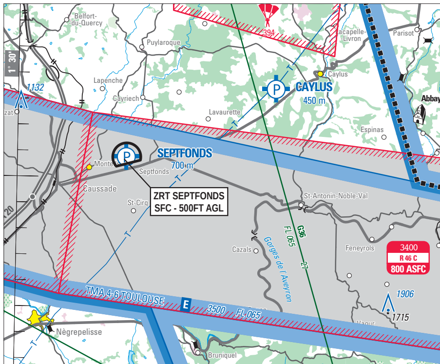
From 1 : 250 000 "Toulouse Région Occitanie" SIA map 2019 1st edition
